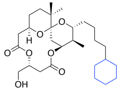
Molecules 2017 , 22 , 631.
