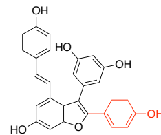
Viniferifuran Antibacterial activity
