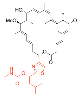
Archazolid F Anticancer activity
