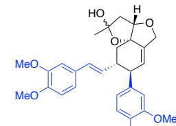
Neovibsanin B Neurite outgrowth promoting activity
