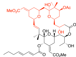
Bryostatin 1 Protein Kinase C activator
