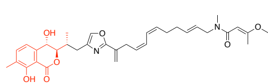
Ajudazol A Respiratory chain inhibitory activity
