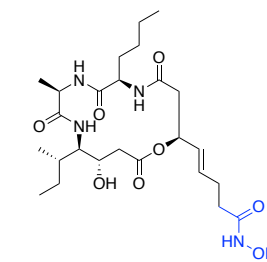
Aplysiatoxin Protein Kinase C activator
