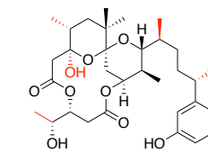
Aplysiatoxin Protein Kinase C activator
