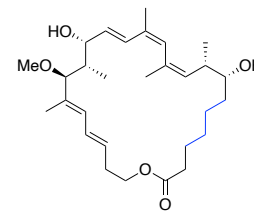
Archazolid JMC 2020, 63, 1684.
