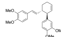
trans-Banglene Neurotogenic activity
