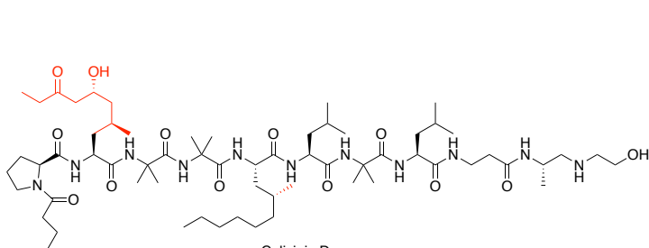
Culicinin D Anticancer activity
