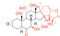
Teccalonolide A Microtubule stabilizer
