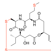
Thailandepsin B HDAC inhibitor
