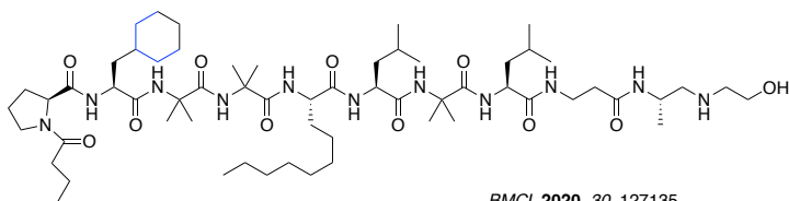
Culicinin D Anticancer activity
