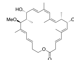
Archazolid JMC 2020, 63, 1684.
