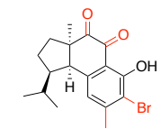
(-)-Hamigeran B Neurite outgrowth inducer
