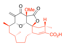
Chrolactomycin Telomerase inhibitor
