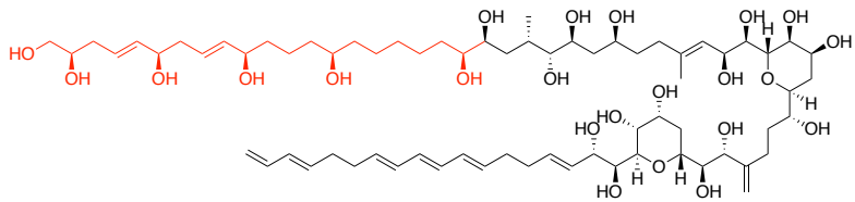
Amphidinol 3 Antifungal activity
