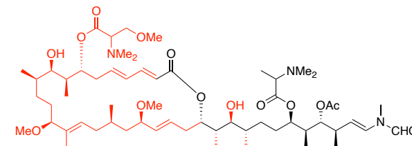
Aplyronine A Actin polymerization inhibitor
