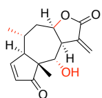
Helenalin NFκB inhibitor
