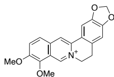
Berberine Antibacterial activity
