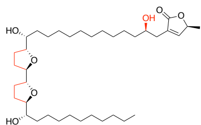
Bullatacin Mitochondrial complex I inhibitor
