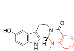
Evodiamine Topoisomerase inhibitor
