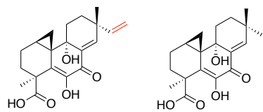
(-)-Myrocin G Antiproliferative activity
