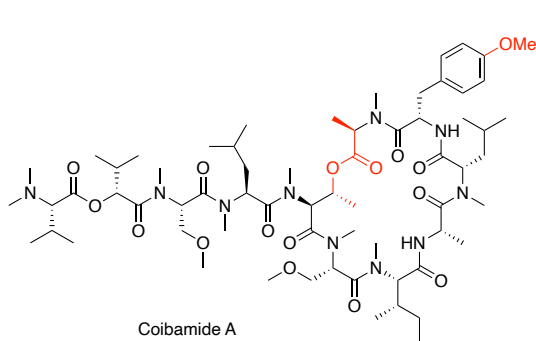
Coibamide A Sec61 translocan inhibitor
