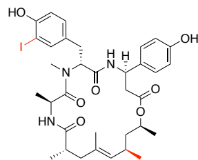
Geodiamolide H Actin fiber stabilizer
