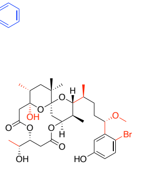
Aplysiatoxin Protein Kinase C activator
