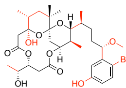
Aplysiatoxin
