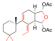
Gracilin A
