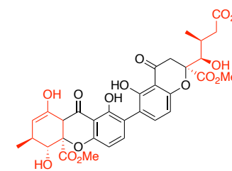
Versixanthone F
