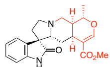
Speciophylline
