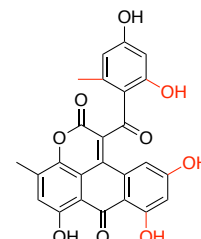
Aspergillide A
