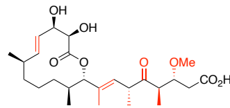
Carolacton
