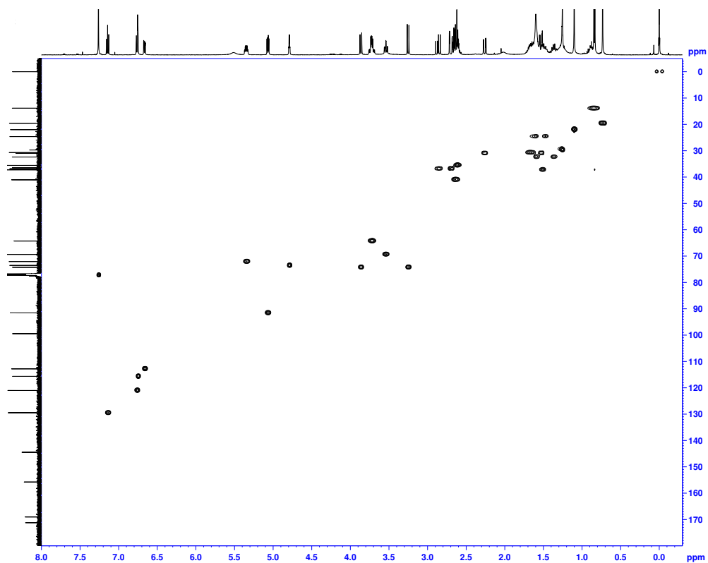
HMBC spectrum of 16 ( ^1\text{H} : 500 MHz, 296.0 K, \text{CDCl}_3 , 0.017 M)
