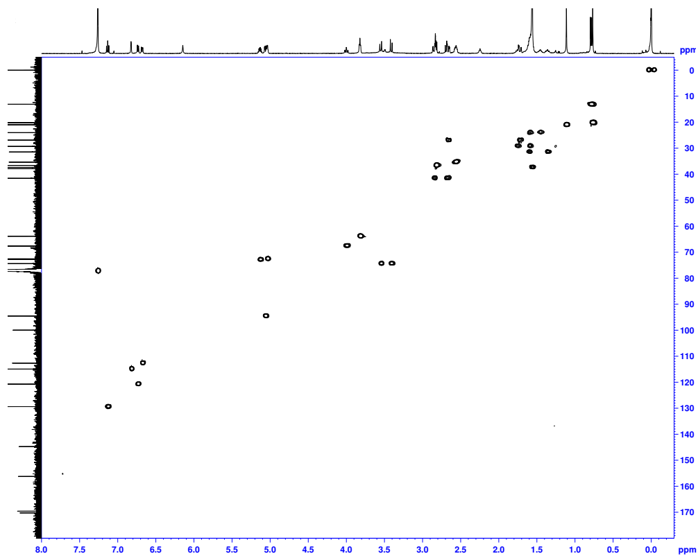
HMBC spectrum of 2 ( ^1\text{H} : 500 MHz, 296.0 K, \text{CDCl}_3 , 0.0026 M)
